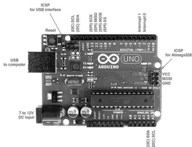
Figure 3.4: Arduino UNO R3 pinouts
