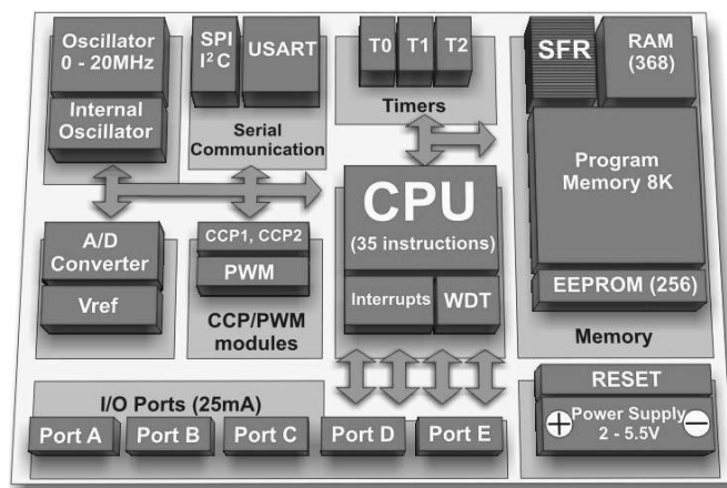
Figure 3.3: Microcontroller architecture [6]
