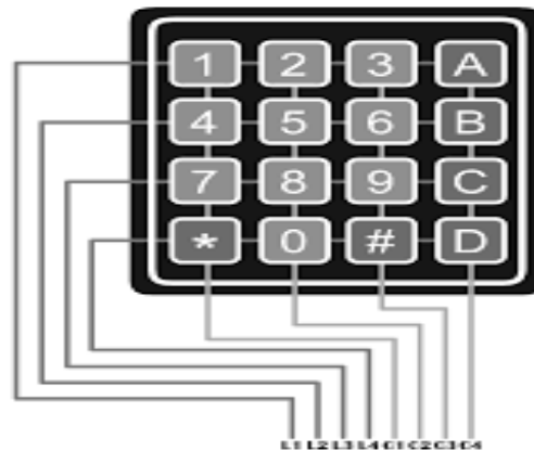
Figure 3.5: 4x4 Matrix keypad
