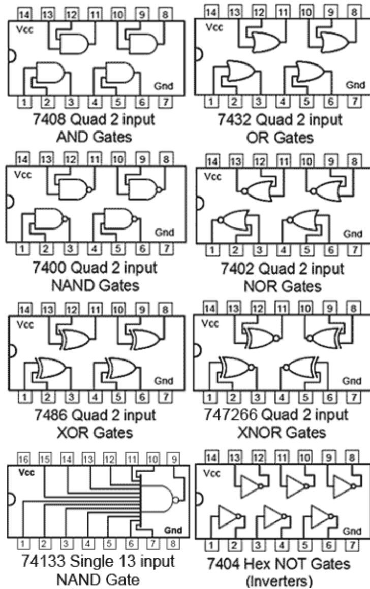
Figure 2.1: 74 Series Logic ICs
