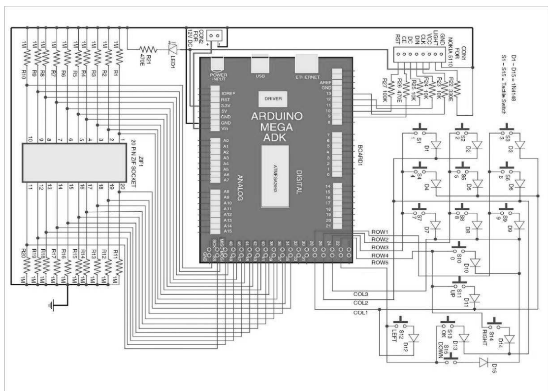
Figure 4.2: Hardware circuit
